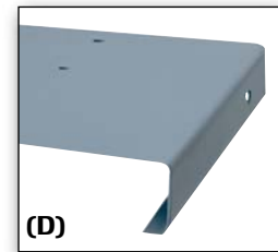
(D) 18-Gauge Traditional flanged shelves afford 750 lb. capacity* for electrical fittings, clamps, bearings, etc.
