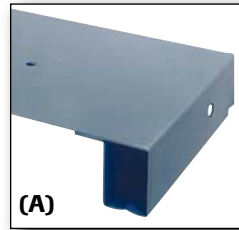
(A) 22-Gauge Medium Duty, Box "W" shelves offer 600 lb. capacity* for storage of aerosols, tools, drills, safety supplies, etc.
