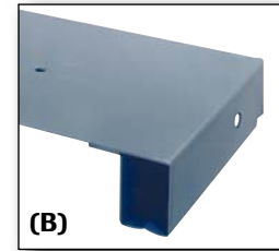
(B) 20-Gauge, Heavy Duty, Box "W" shelves provide 900 lb. capacity* to hold grinders, wheels, gears, sprockets, and other similar articles.
